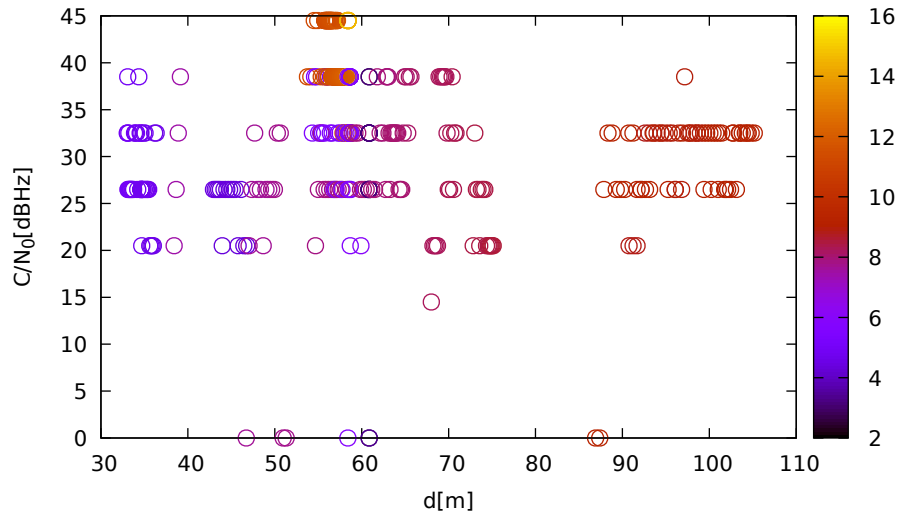
C/N 0 vs distance (LeicaGS15 at C 1 for G27 at L2)
