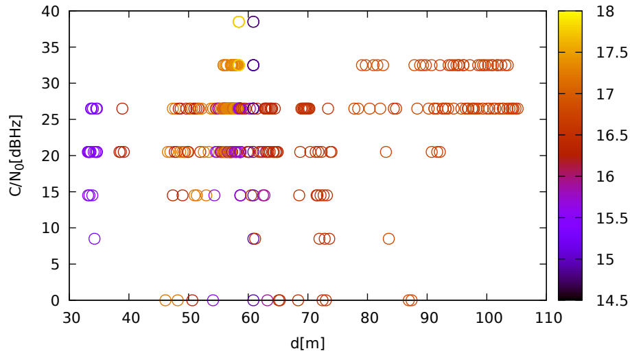
C/N 0 vs distance (LeicaGS15 at C 1 for G28 at L2)
