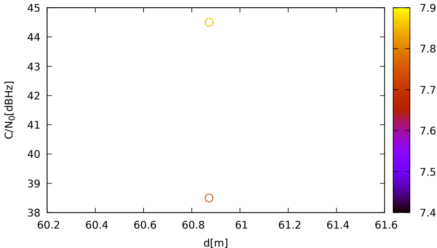
C/N 0 vs distance (LeicaGS15 at C 1 for G31 at L2)
