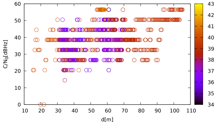
C/N 0 vs distance (LeicaGS15 at C 1 for G32 at L2)
