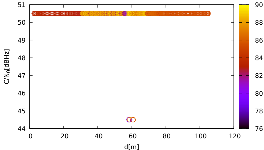
C/N 0 vs distance (LeicaGS15 at C 1 for R07 at L2)
