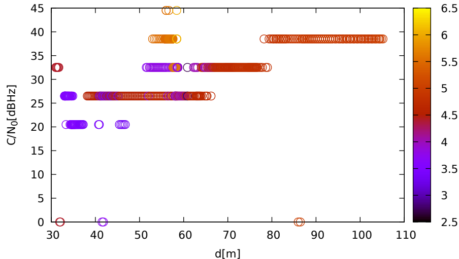
C/N 0 vs distance (LeicaGS15 at C 1 for R14 at L2)
