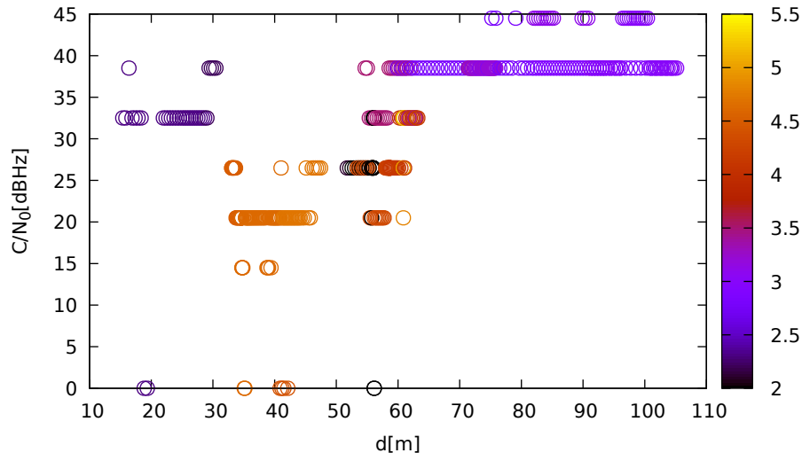
C/N 0 vs distance (LeicaGS15 at C 1 for R15 at L2)
