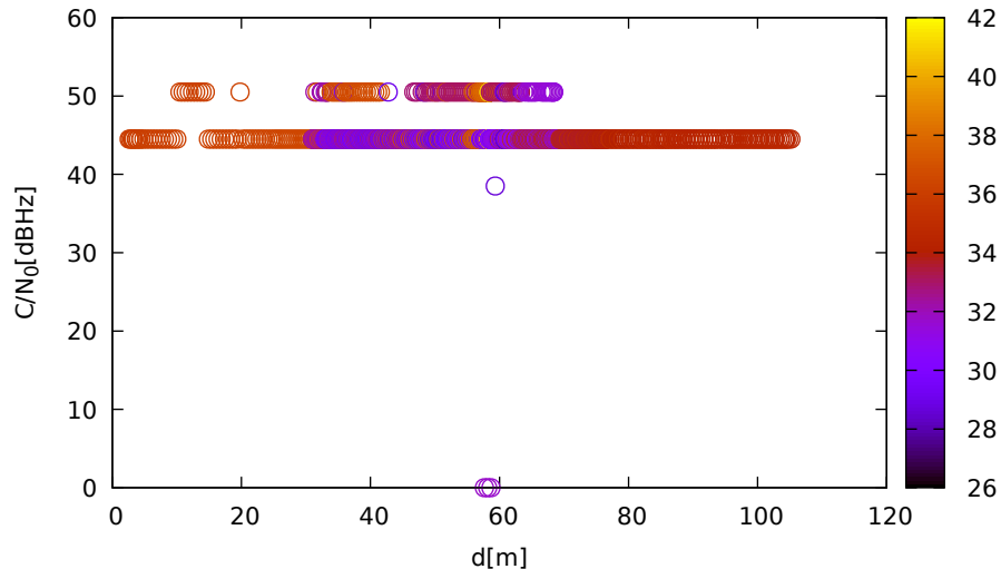
C/N 0 vs distance (LeicaGS15 at C 1 for R21 at L2)
