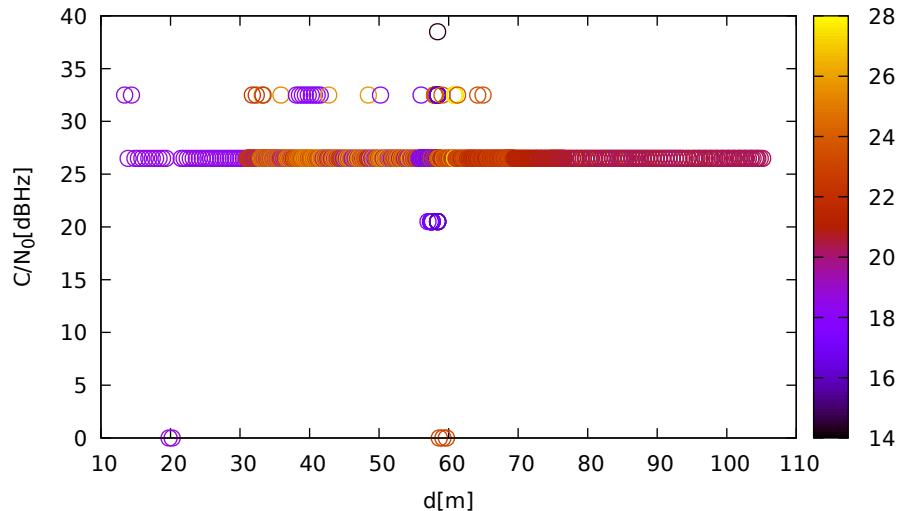
C/N 0 vs distance (LeicaGS15 at C 1 for R23 at L2)
