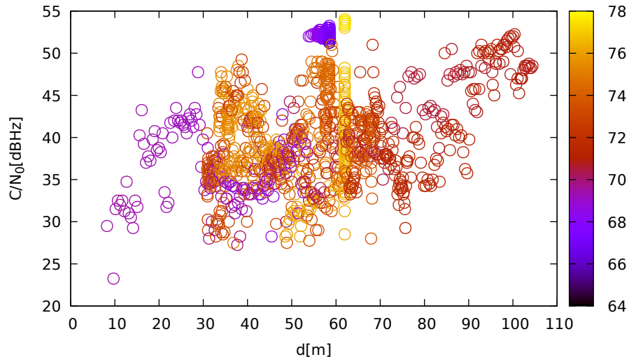
C/N 0 vs distance (LeicaGS18 at C 1 for G01 at L2)
