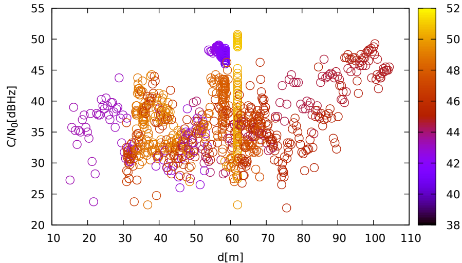
C/N 0 vs distance (LeicaGS18 at C 1 for G03 at L2)
