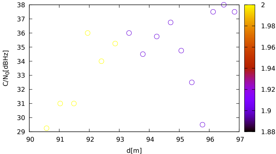
C/N 0 vs distance (LeicaGS18 at C 1 for G04 at L2)
