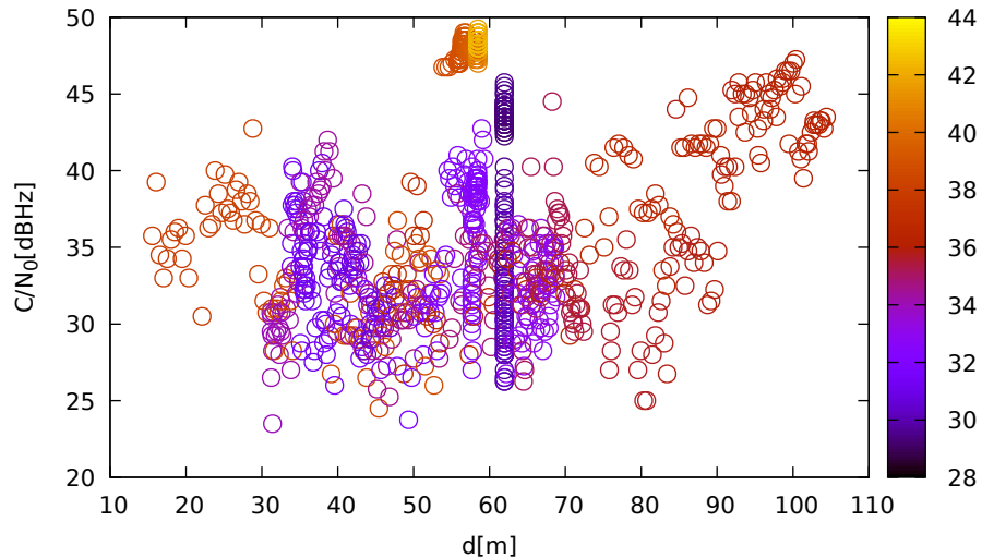
C/N 0 vs distance (LeicaGS18 at C 1 for G08 at L2)
