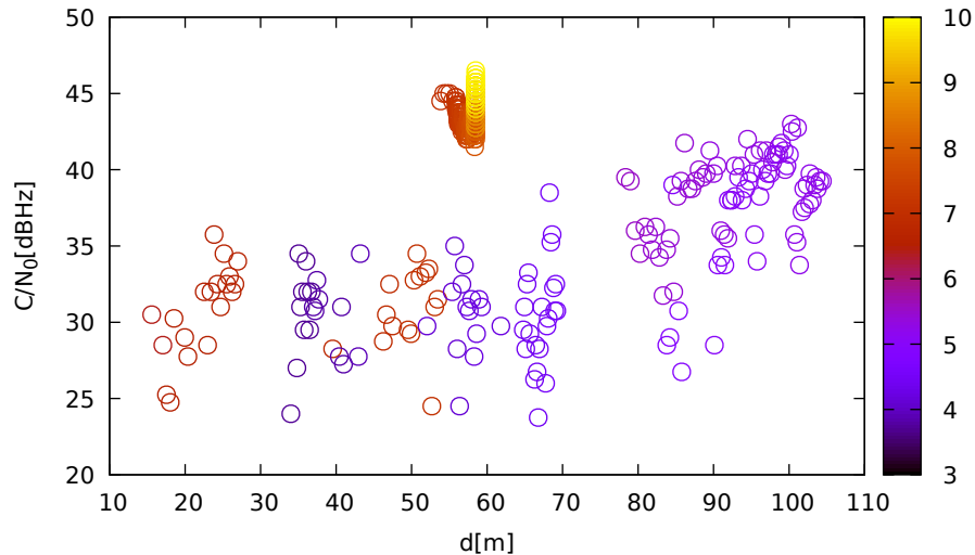
C/N 0 vs distance (LeicaGS18 at C 1 for G10 at L2)
