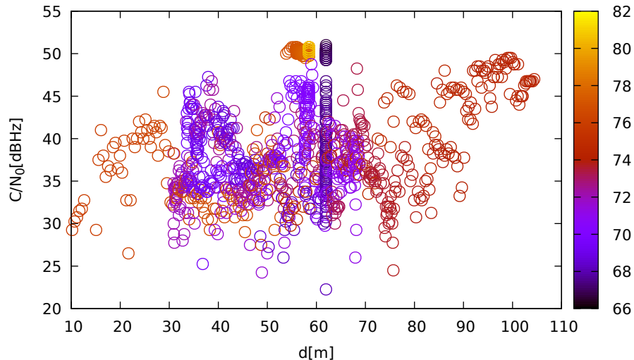
C/N 0 vs distance (LeicaGS18 at C 1 for G11 at L2)
