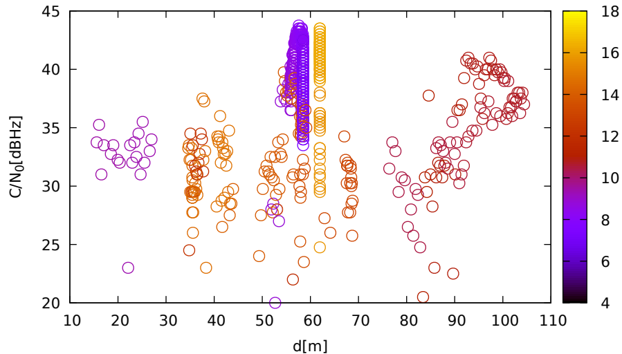
C/N 0 vs distance (LeicaGS18 at C 1 for G17 at L2)
