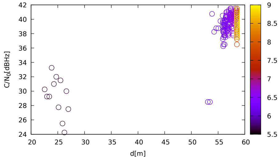
C/N 0 vs distance (LeicaGS18 at C 1 for G21 at L2)
