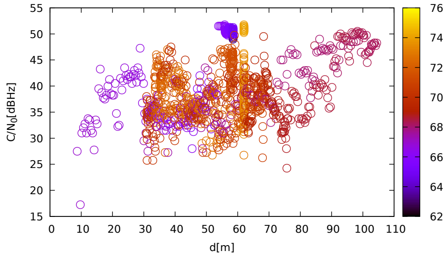
C/N 0 vs distance (LeicaGS18 at C 1 for G22 at L2)
