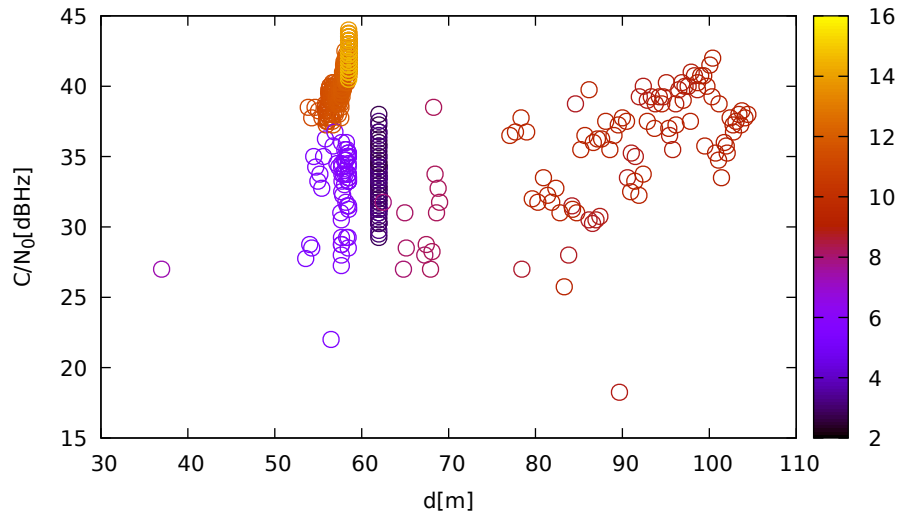
C/N 0 vs distance (LeicaGS18 at C 1 for G27 at L2)
