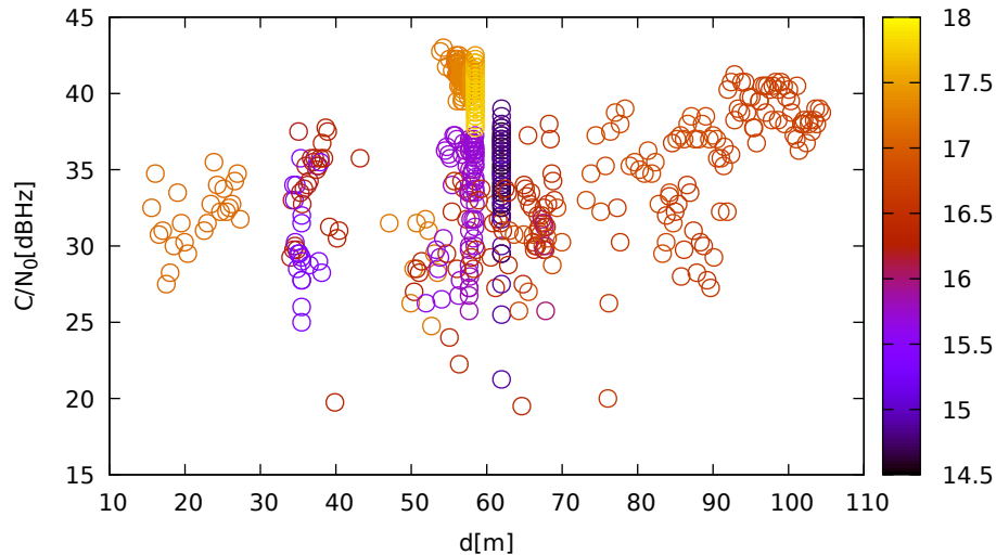
C/N 0 vs distance (LeicaGS18 at C 1 for G28 at L2)
