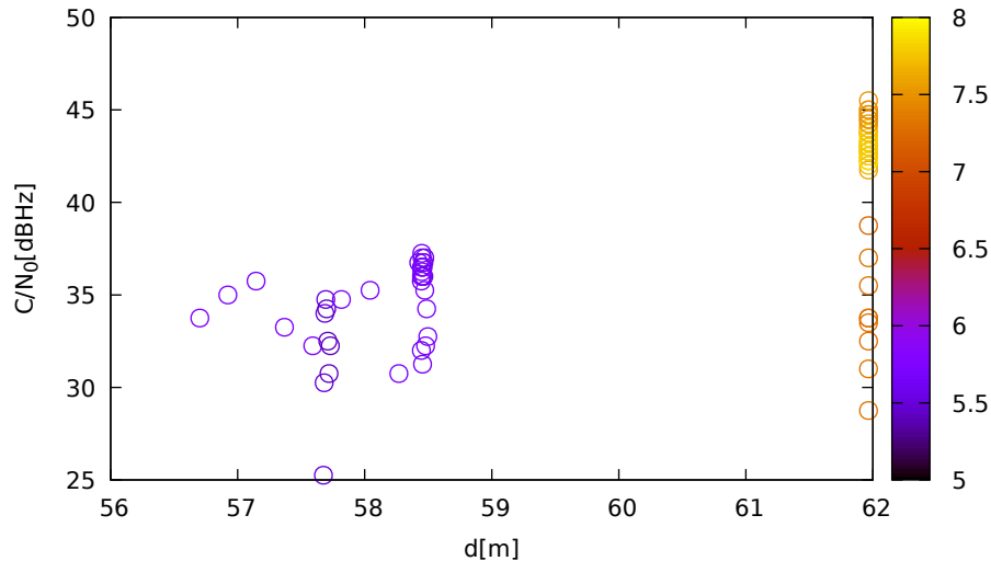
C/N 0 vs distance (LeicaGS18 at C 1 for G31 at L2)
