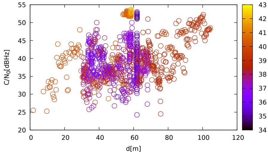
C/N 0 vs distance (LeicaGS18 at C 1 for G32 at L2)
