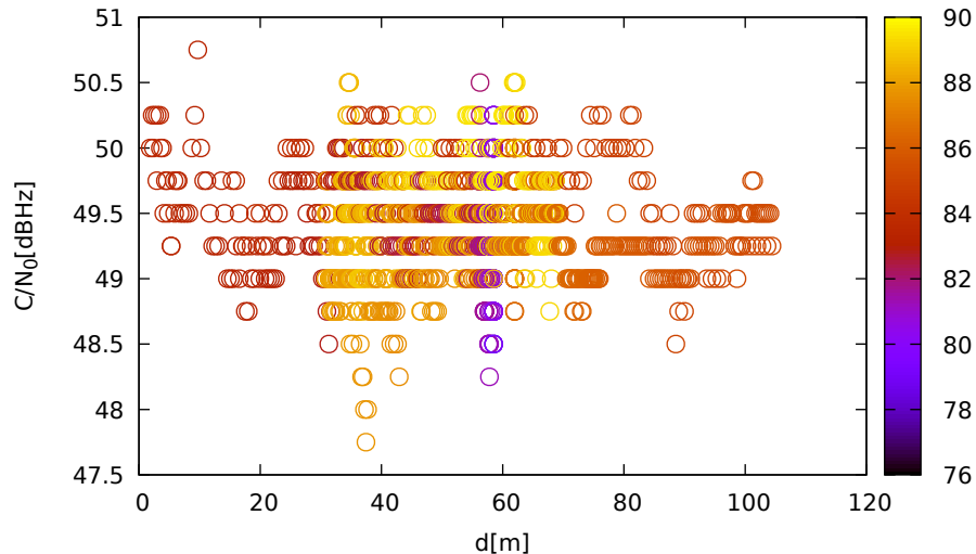
C/N 0 vs distance (LeicaGS18 at C 1 for R07 at L2)
