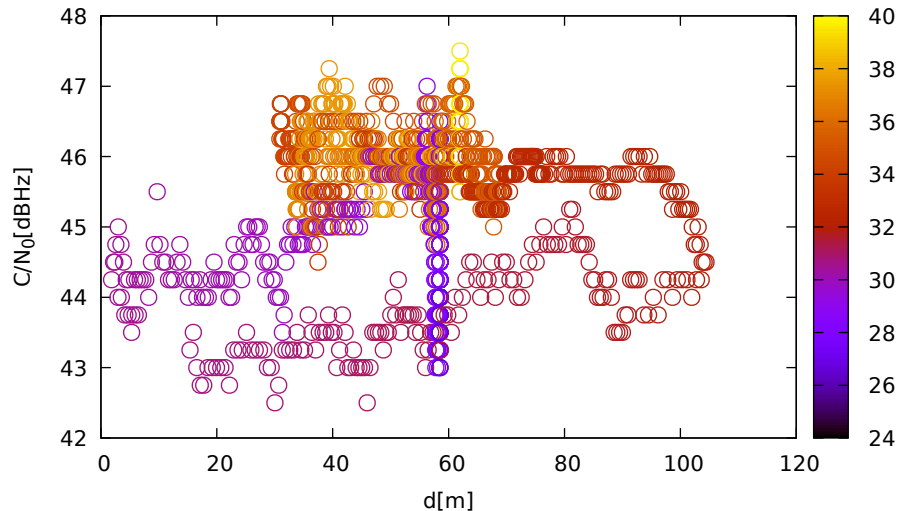
C/N 0 vs distance (LeicaGS18 at C 1 for R08 at L2)
