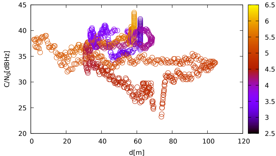
C/N 0 vs distance (LeicaGS18 at C 1 for R14 at L2)
