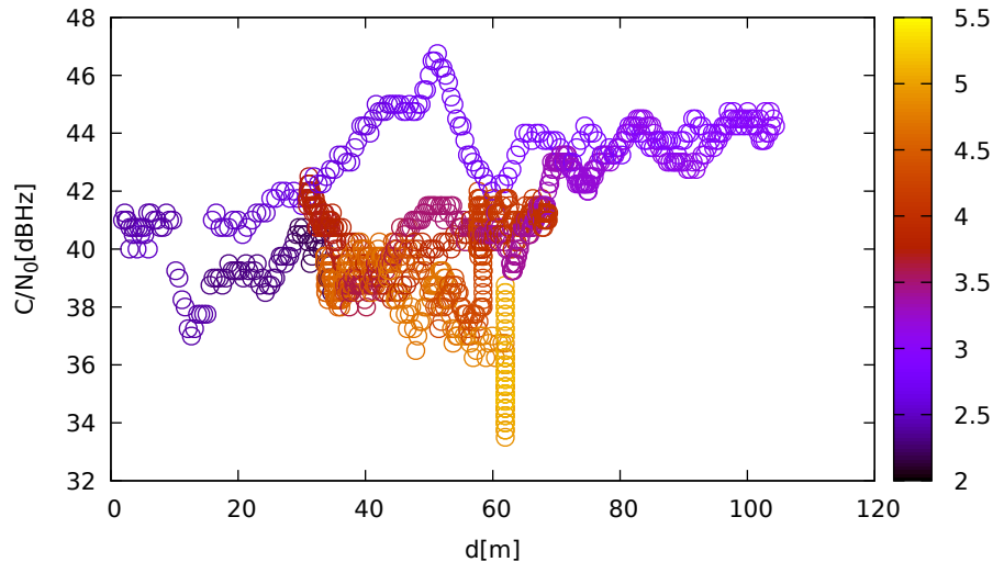
C/N 0 vs distance (LeicaGS18 at C 1 for R15 at L2)
