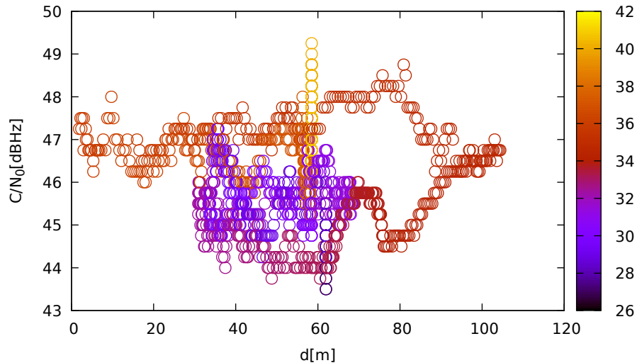
C/N 0 vs distance (LeicaGS18 at C 1 for R21 at L2)
