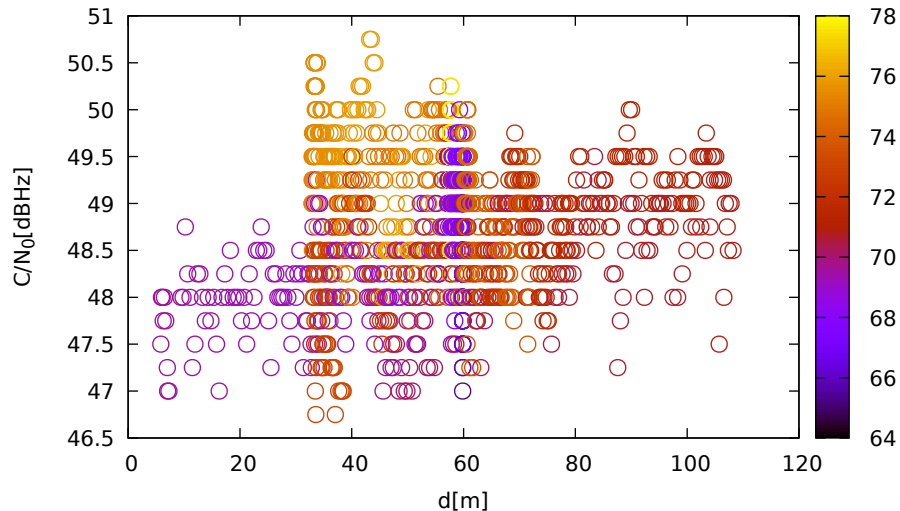
C/N 0 vs distance (TrimbleR8s at C 1 for G01 at L2)
