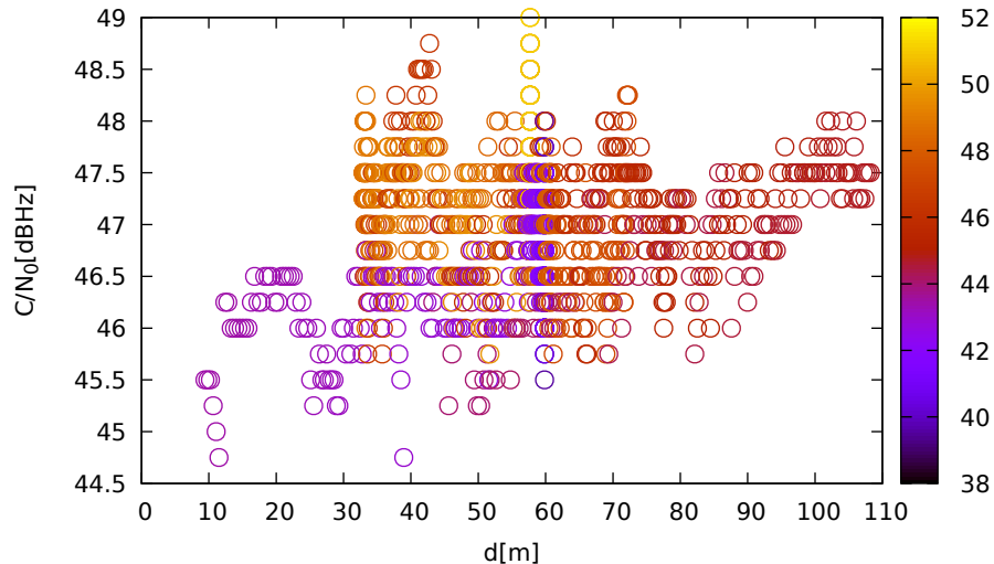
C/N 0 vs distance (TrimbleR8s at C 1 for G03 at L2)
