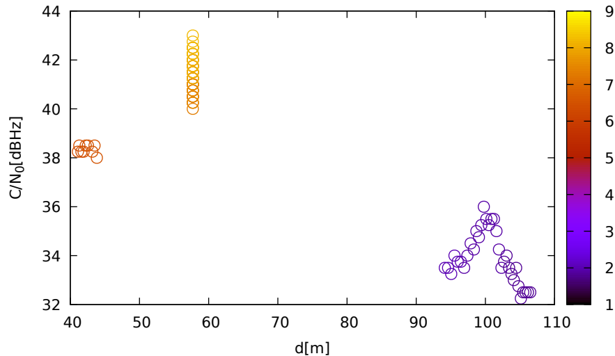
C/N 0 vs distance (TrimbleR8s at C 1 for G04 at L2)
