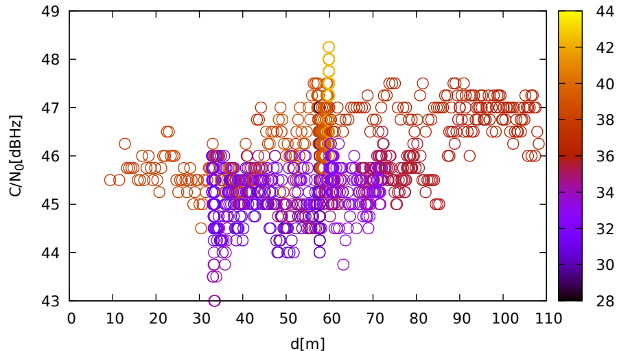
C/N 0 vs distance (TrimbleR8s at C 1 for G08 at L2)
