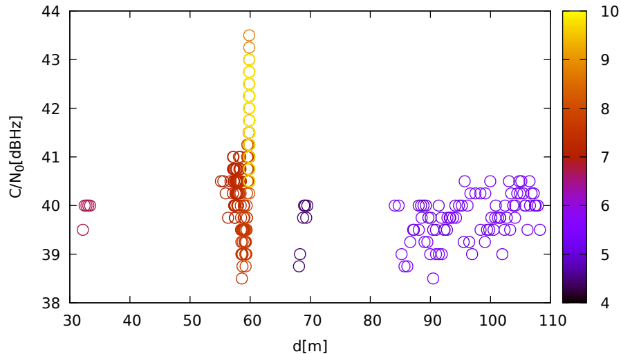
C/N 0 vs distance (TrimbleR8s at C 1 for G10 at L2)
