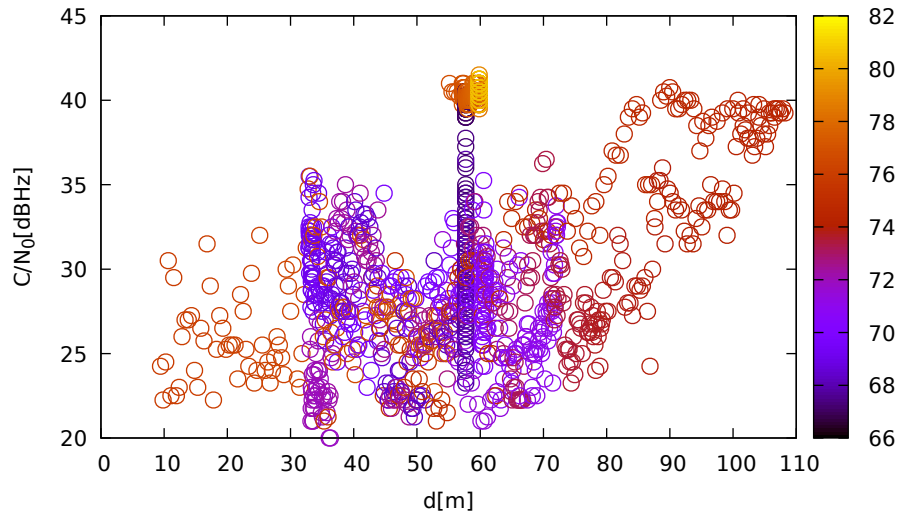
C/N 0 vs distance (TrimbleR8s at C 1 for G11 at L2)
