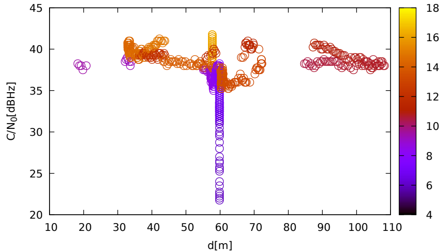
C/N 0 vs distance (TrimbleR8s at C 1 for G17 at L2)
