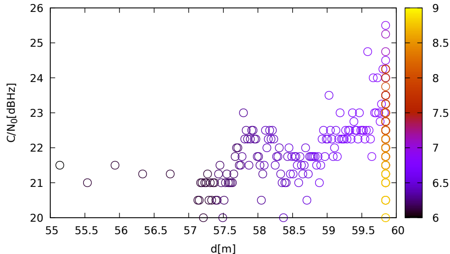
C/N 0 vs distance (TrimbleR8s at C 1 for G21 at L2)
