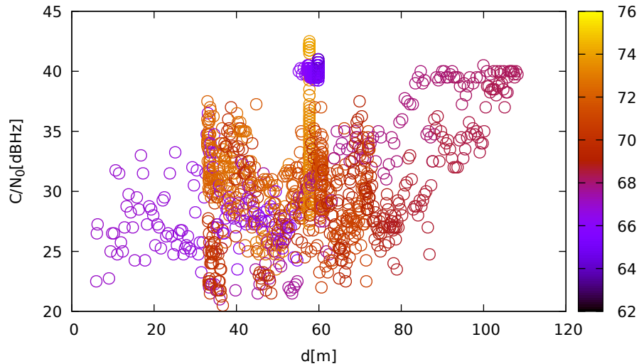
C/N 0 vs distance (TrimbleR8s at C 1 for G22 at L2)
