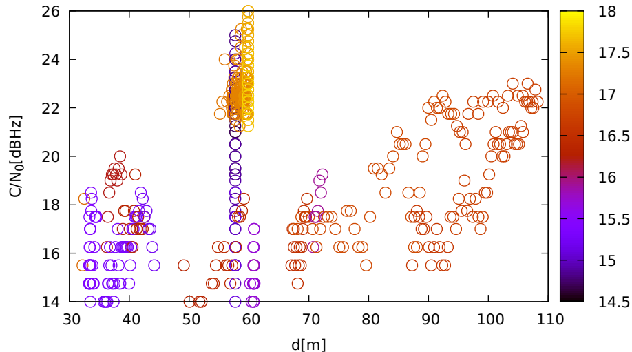
C/N 0 vs distance (TrimbleR8s at C 1 for G28 at L2)
