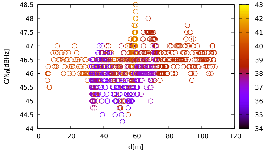
C/N 0 vs distance (TrimbleR8s at C 1 for G32 at L2)
