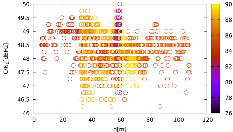
C/N 0 vs distance (TrimbleR8s at C 1 for R07 at L2)
