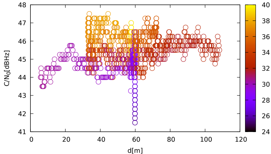
C/N 0 vs distance (TrimbleR8s at C 1 for R08 at L2)
