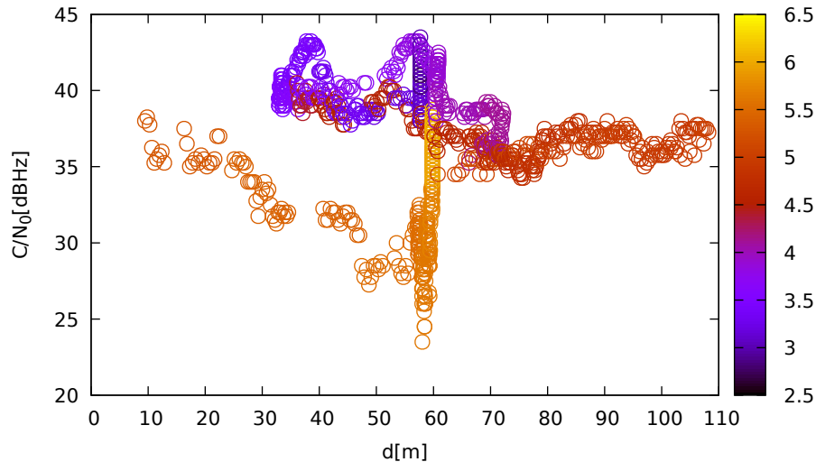
C/N 0 vs distance (TrimbleR8s at C 1 for R14 at L2)
