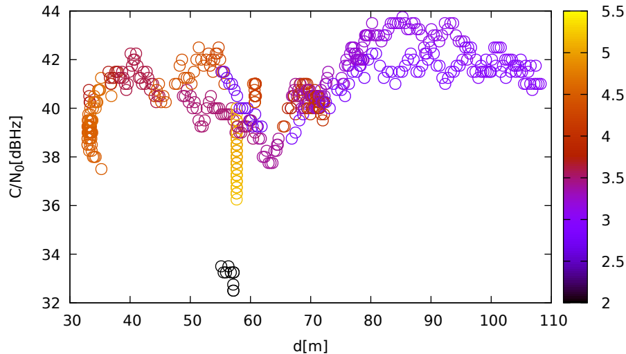
C/N 0 vs distance (TrimbleR8s at C 1 for R15 at L2)
