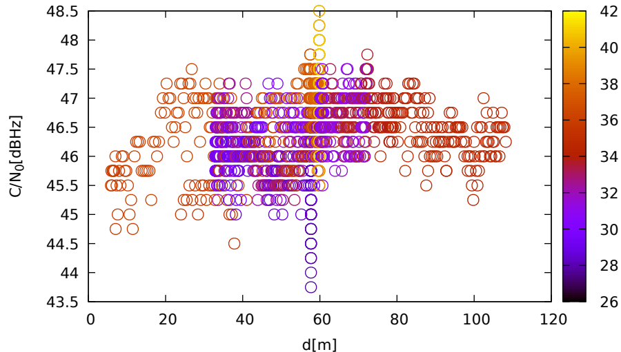
C/N 0 vs distance (TrimbleR8s at C 1 for R21 at L2)
