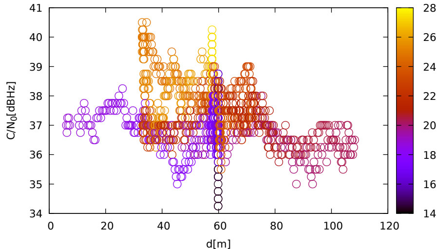
C/N 0 vs distance (TrimbleR8s at C 1 for R23 at L2)
