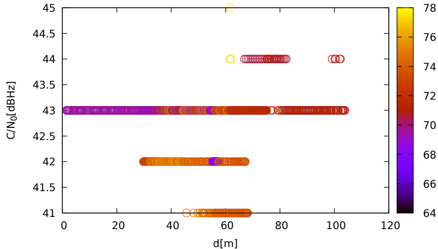
C/N 0 vs distance (ublox9 at C 1 for G01 at L2)
