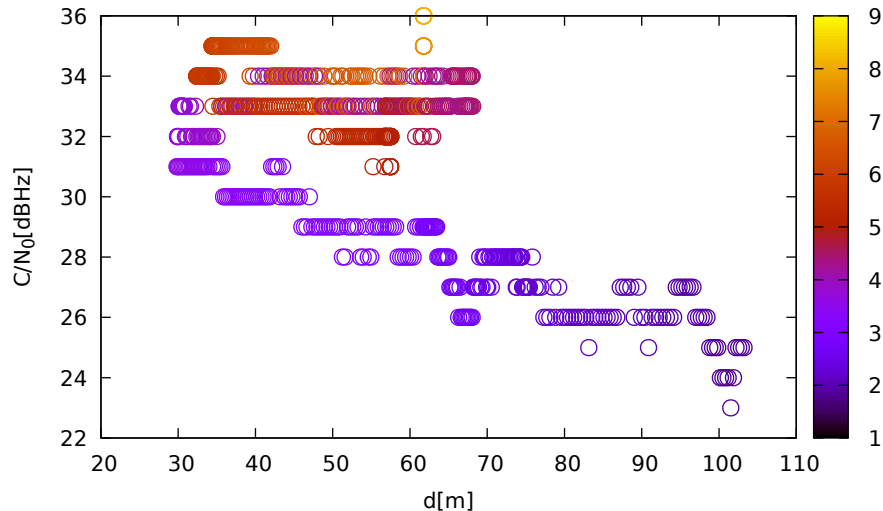
C/N 0 vs distance (ublox9 at C 1 for G04 at L2)
