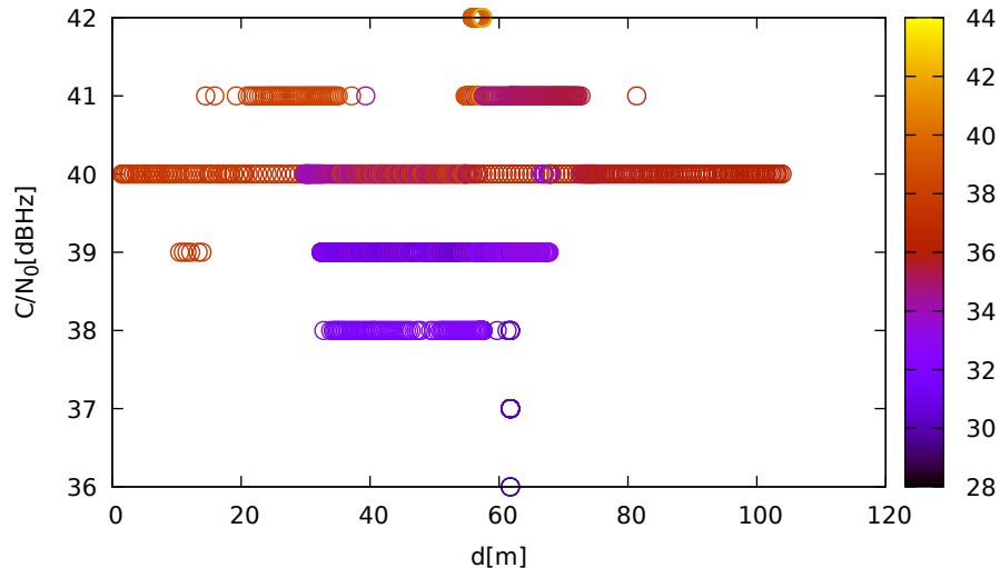
C/N 0 vs distance (ublox9 at C 1 for G08 at L2)
