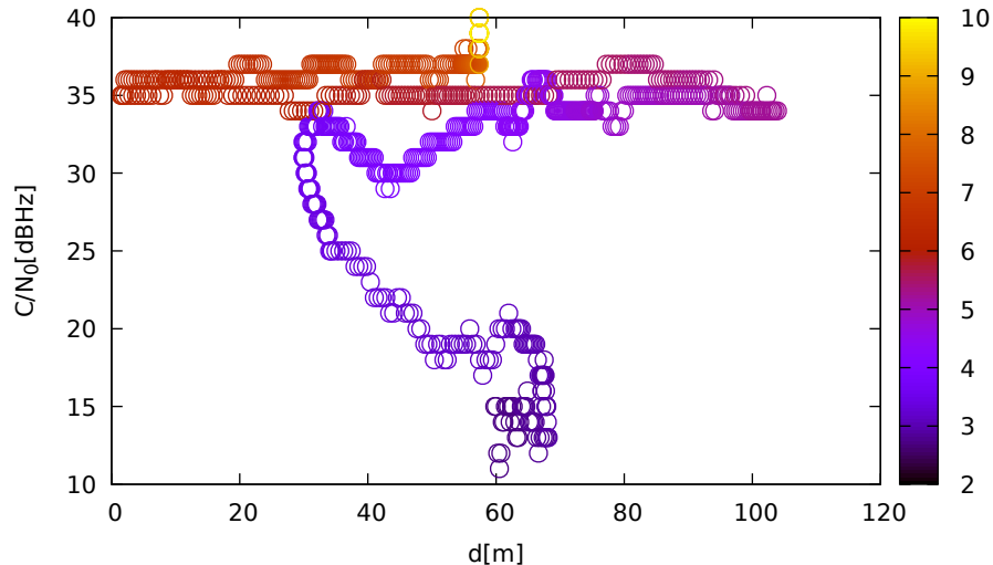
C/N 0 vs distance (ublox9 at C 1 for G10 at L2)
