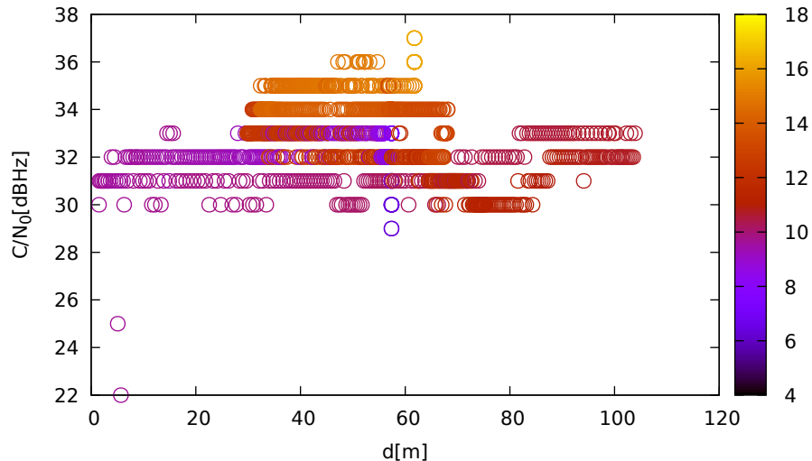
C/N 0 vs distance (ublox9 at C 1 for G17 at L2)
