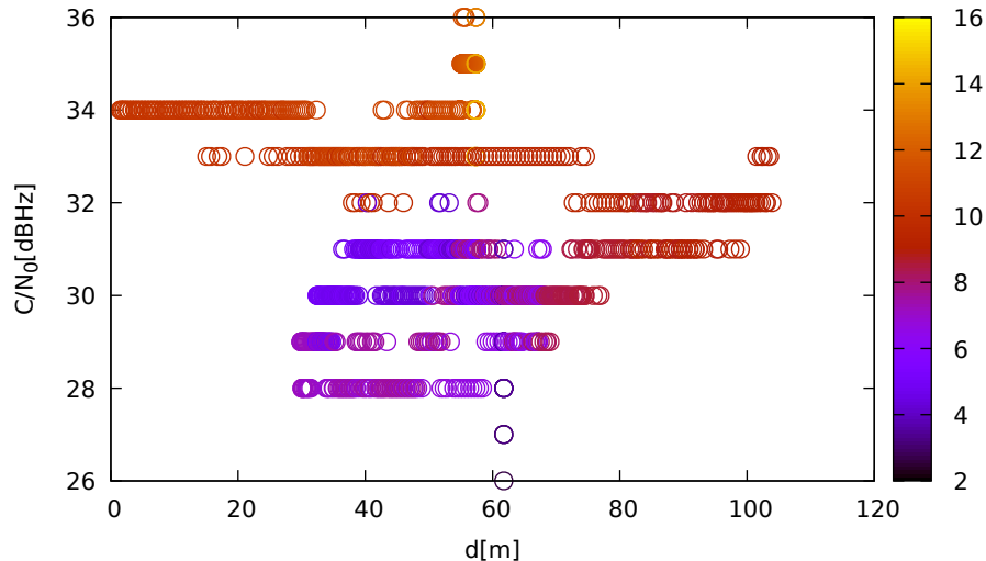
C/N 0 vs distance (ublox9 at C 1 for G27 at L2)
